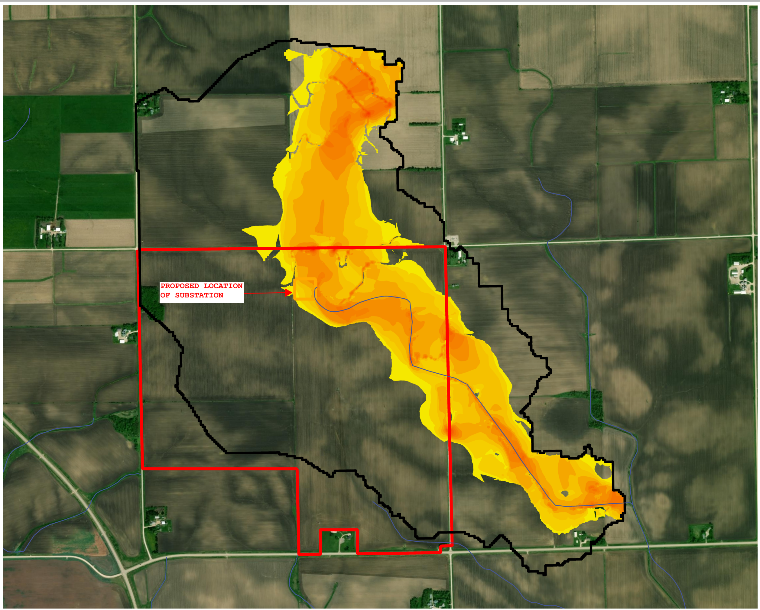
Figure 3: Max Velocity Map (fps) 100yr 24hr storm
